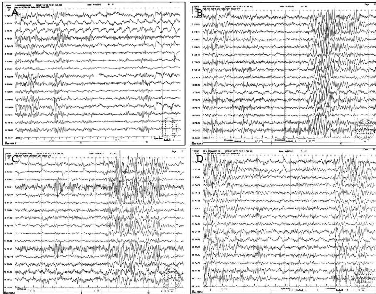
Figure 1. Electroencephalogram (EEG) study epochs belonging to case 1
