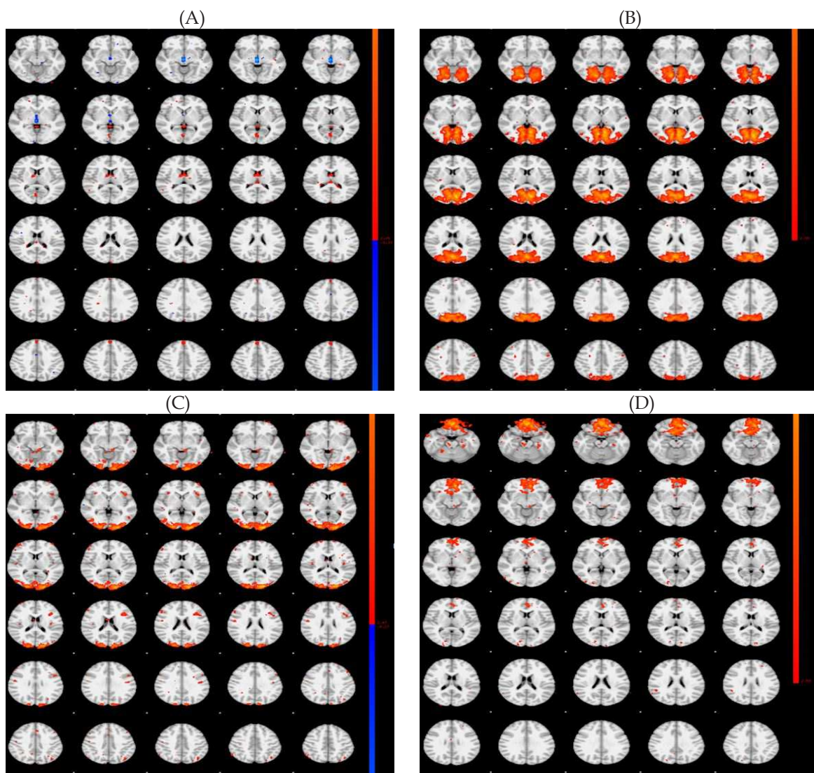
Figure 2. fMRI group level activation map for BOLD response during off or minimally presented headache based on the self scored VAS using (A) and during maximal headache episodes (B, C and D). Functional data were analyzed using scripts in FMRIB's Software Library (FSL). The analyzed data were used for a group-level activation map, through the mixed-level model. The voxel wise paired t-test was employed to distinguish possible differences in activation during off-headache and maximal headache state fMRI assessment. During headache bouts, group-level activation map fMRI, revealed a markedly increased BOLD signal in bilateral occipital regions (B, C) and also modest fronto-polar BOLD signal increase(D). These changes were not seen in off-headache conditions (A).
