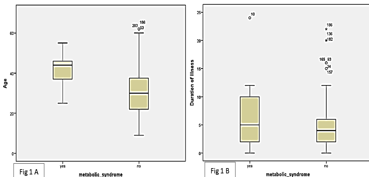
Figure 1. A) Box and whisker plot showing median (thick black line) and interquartile range (IQR) with whisker showing 95% confidence interval (CI) for correlation between age and metabolic syndrome in patients with migraine; B) Box and whisker plot showing median (thick black line) and IQR with whisker showing 95% CI for correlation between duration of illness and metabolic syndrome in patients with migraine
